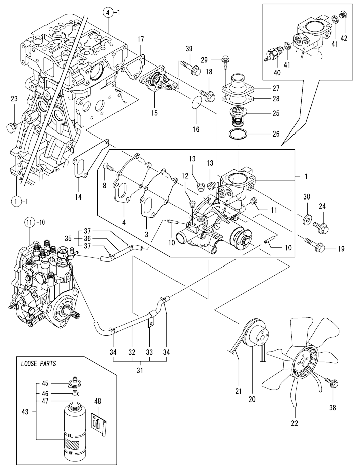
Fig.10. COLING WATER SYSTEM
