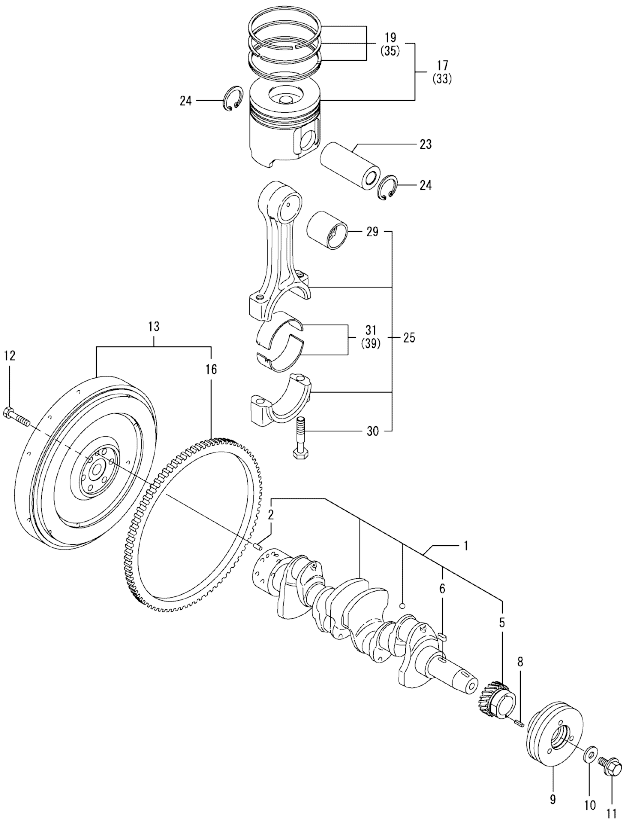
Fig.8. CRANKSHAFT & PISTON
