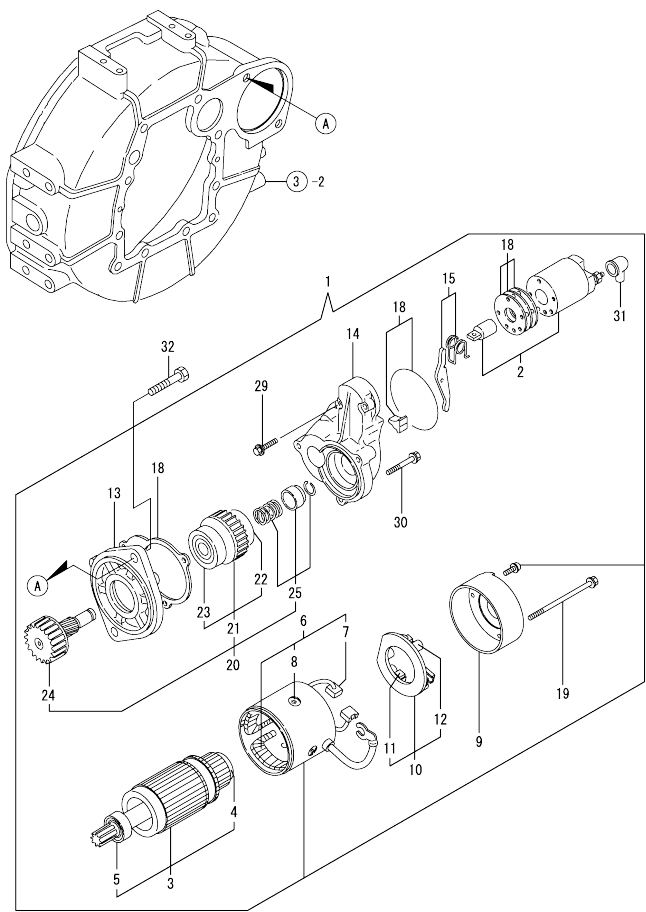
Fig.14. STARTING MOTOR
